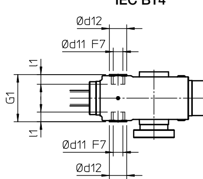
Rear attachment BUSHES Config.3
